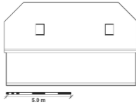
Rear Elevation
